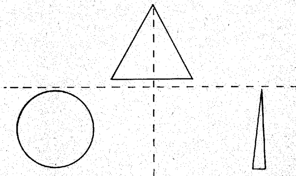
FIG.—Week's Theory of Round and Sharp Type.
